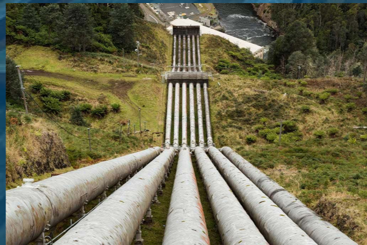
Penstock
