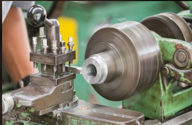
Lathe
